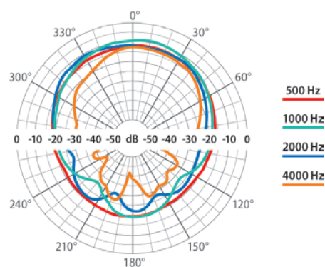
Circular chart of directional characteristic – horizontal:
