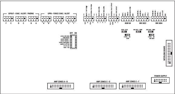
Internal connections
